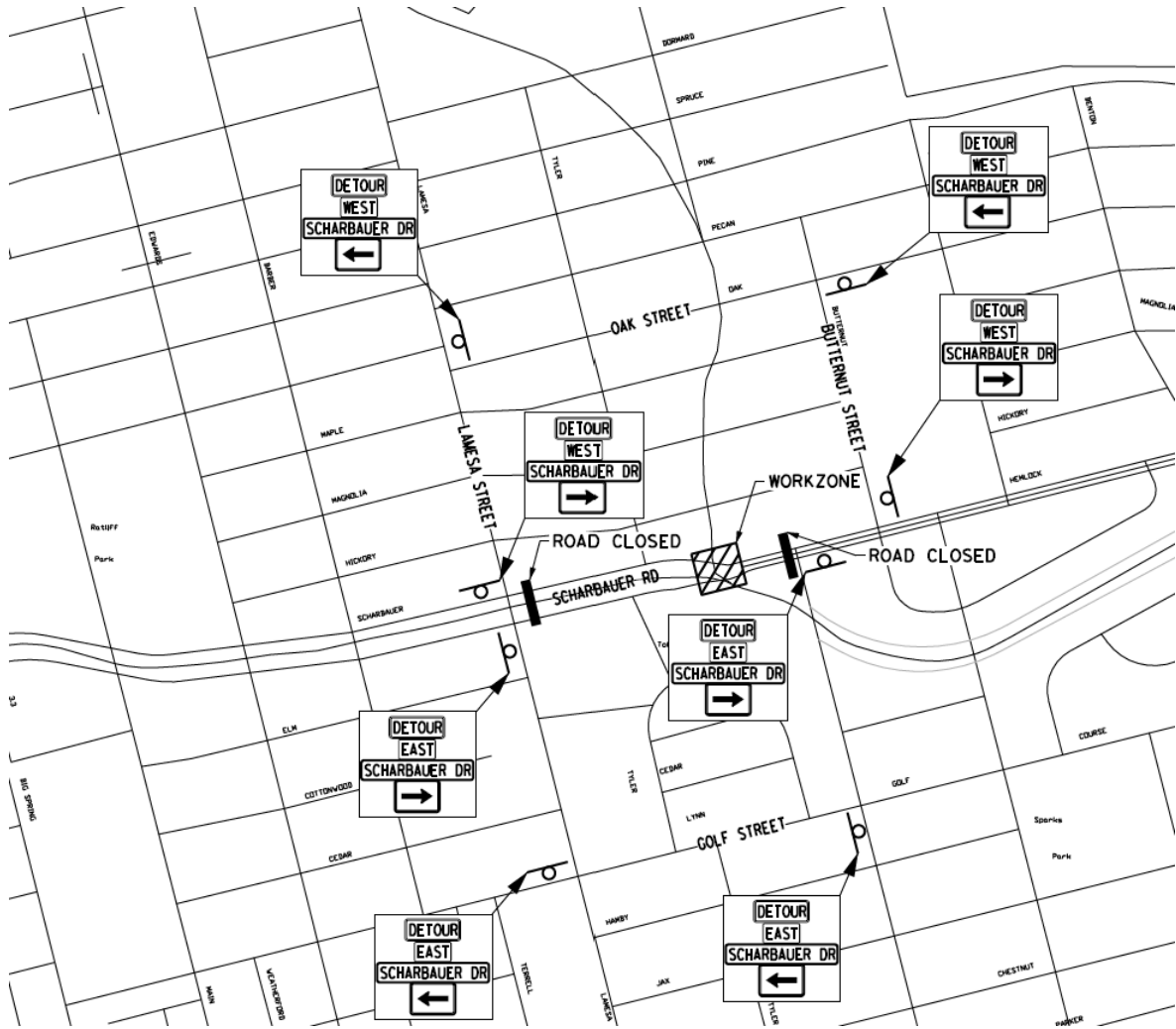
Figure 2 – Scharbauer Drive at Midland Draw Detour Layout
