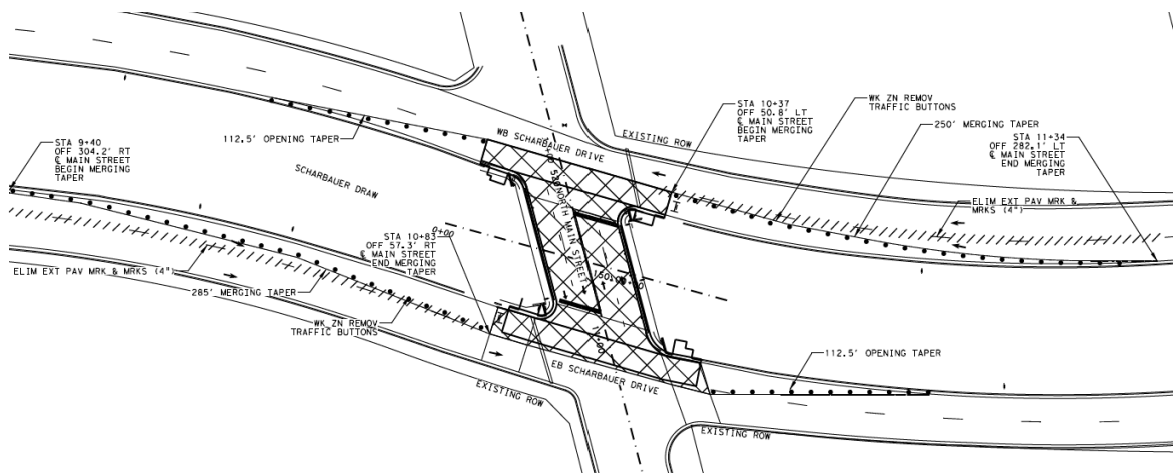
Figure 1 - Main Street at Scharbauer Draw Closure
